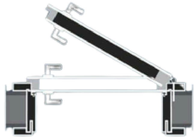
Door opens to the Right
